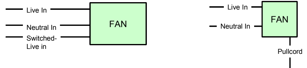
Wiring Diagram for Digital 400HT
