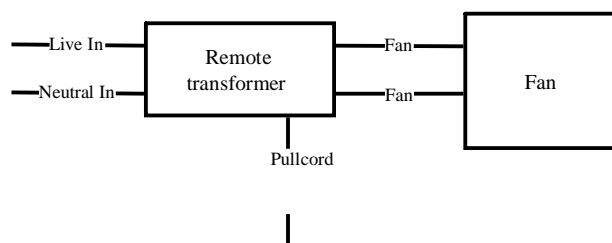
Wiring Diagram for Sensortronic D1007
